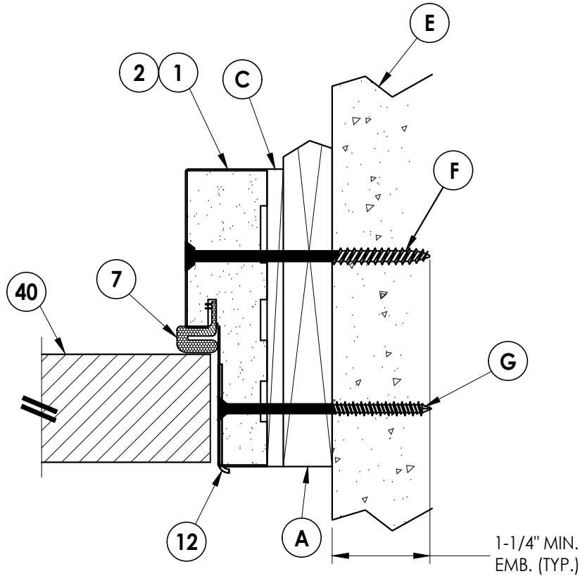
2 4 HORIZONTAL CROSS SECTION Shown w/ 1X Buck Outswing shown (Inswing similar)
