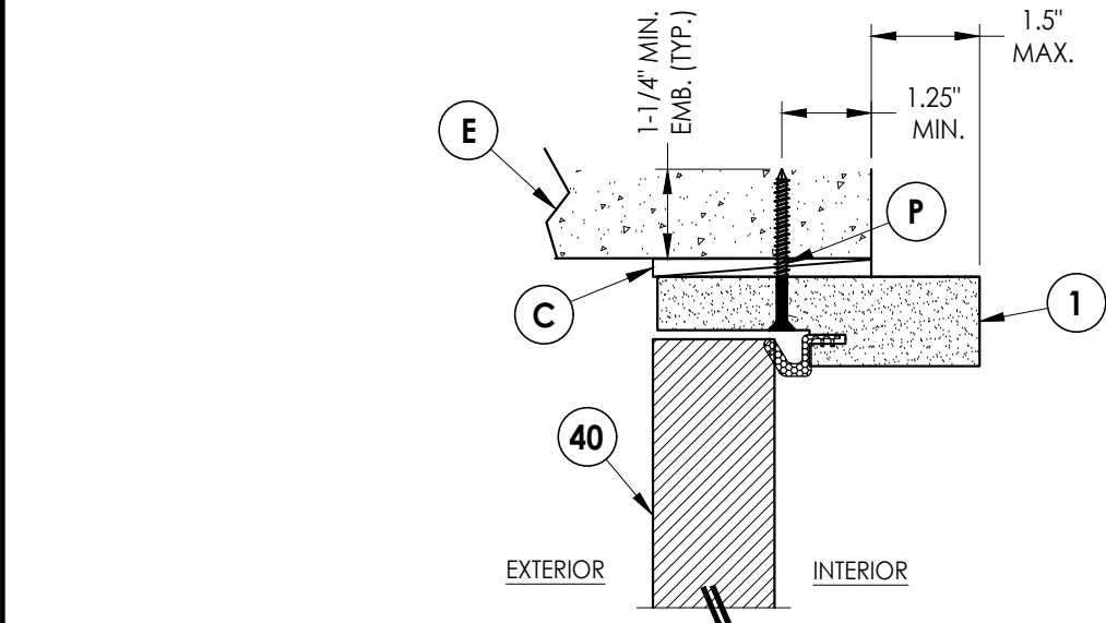
5 VERTICAL CROSS SECTION 7 Shown Direct to Masonry Outswing only w/ 4-9/16" jamb
