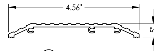
30 ADA THRESHOLD DLP Industries
