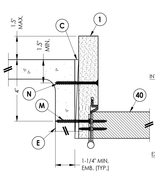
3 HORIZONTAL CROSS SECTION 7 Shown Direct to Masonry Outswing only w/ 6-9/16" jamb
