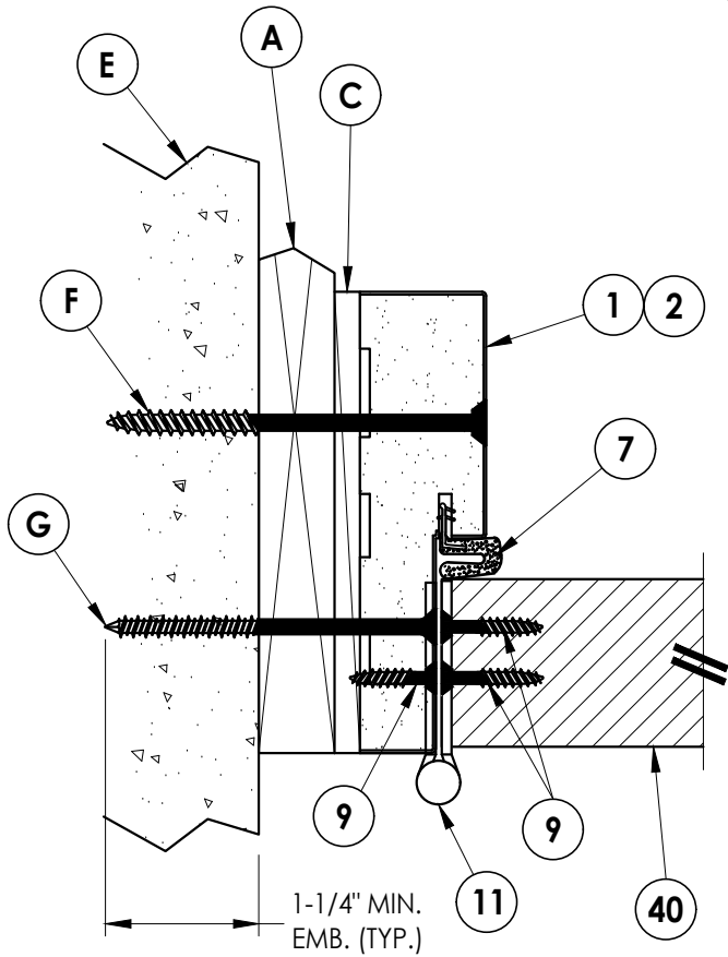
1 4 HORIZONTAL CROSS SECTION Shown w/ 1X Buck Outswing shown (Inswing similar)
