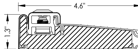
20 INSWING THRESHOLD
